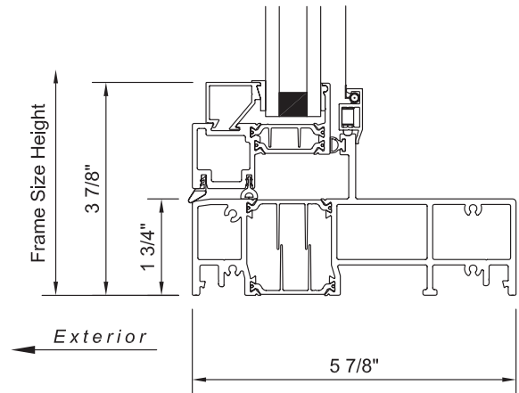
series 7660 awning and series 7670 casement window head - equal leg block high frame
